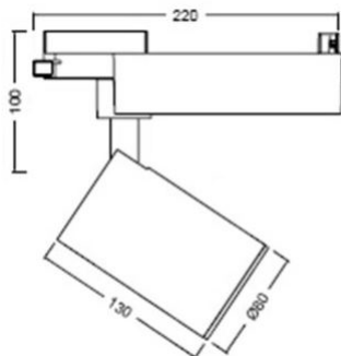
PIL 20W 36°/60°
