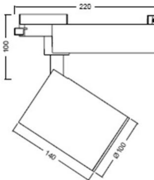
PIL 40W 36°/60°
