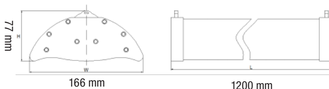
TEGRA High 120W (120cm)
