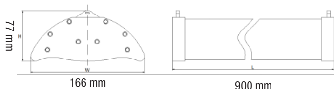
TEGRA High 120W (90cm)
